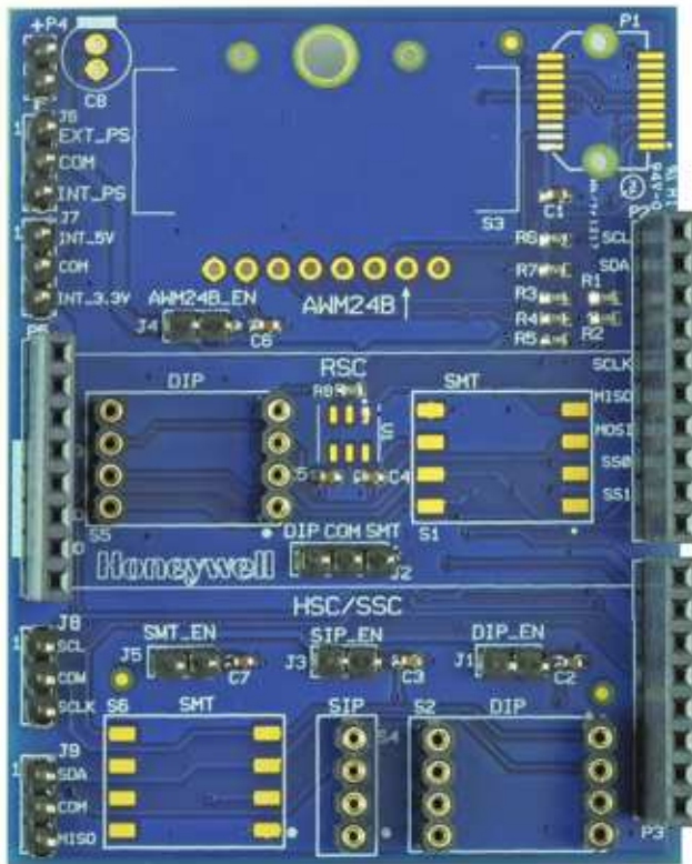
Figure D1. SEK001 Board Layout (Note: The AWM24B set of receiving sockets is not currently used.)
