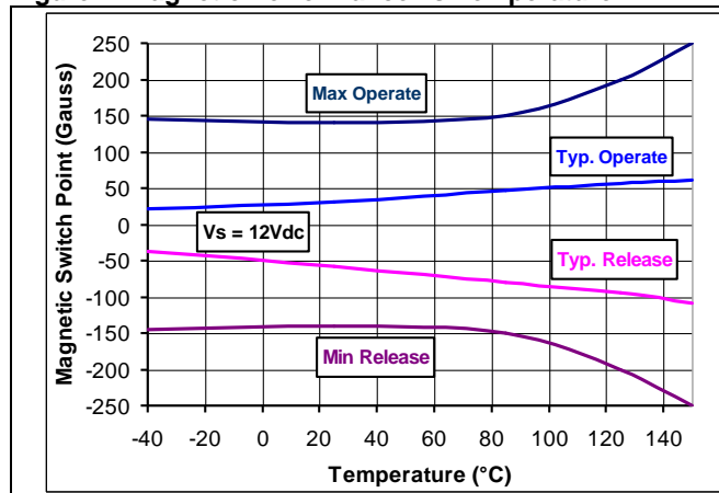
Figure 1. Magnetic Performance vs Temperature
