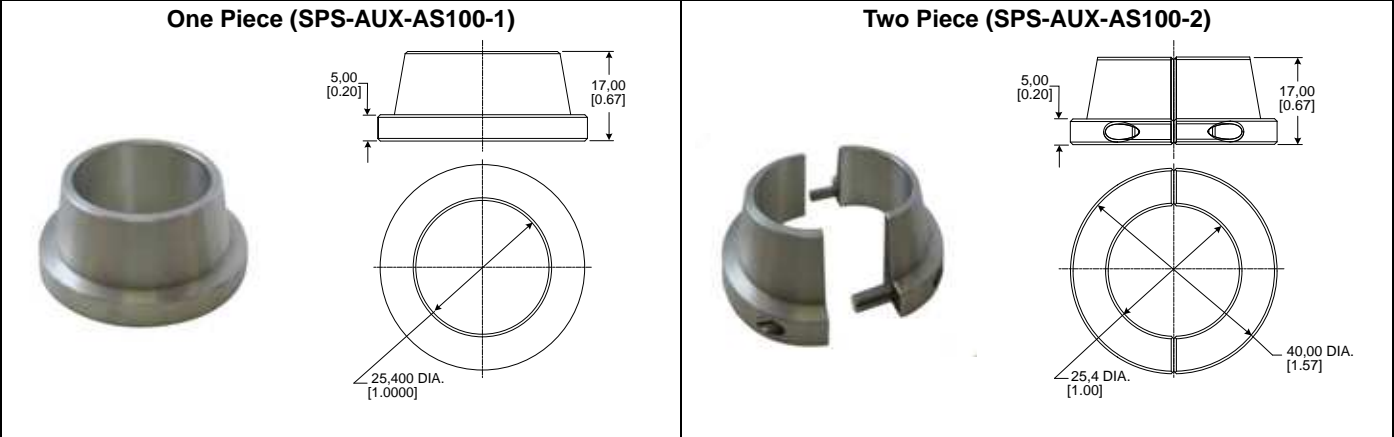
Figure 3. Assembly Tools
