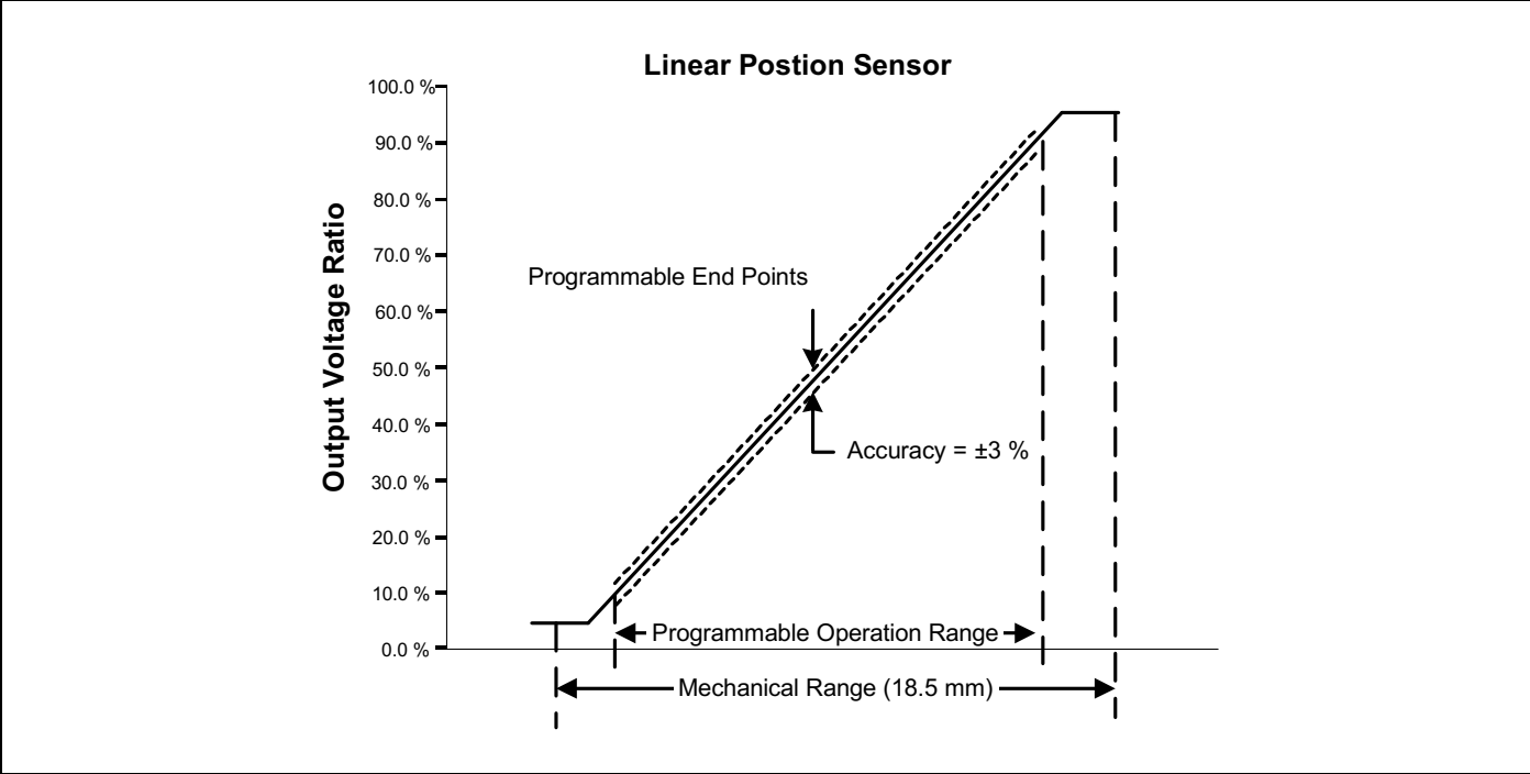
FIGURE 1. OUTPUT VOLTAGE VS POSITION
