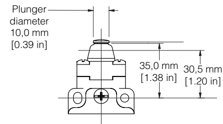
Figure 4. GXA Series Pin Plunger Dimensions
