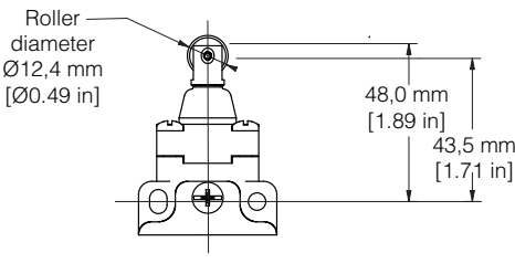
Figure 5. GXA Series Roller Plunger Dimensions
