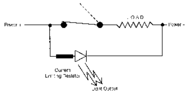
Figure 18. Wiring Diagram 3
