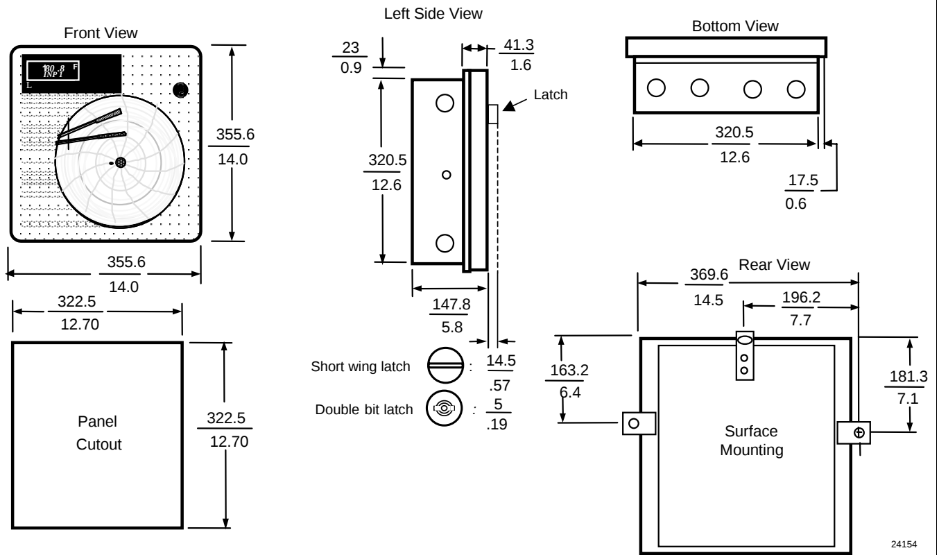
Figure 2—DR4300 Recorder Dimensions—For Reference Only
